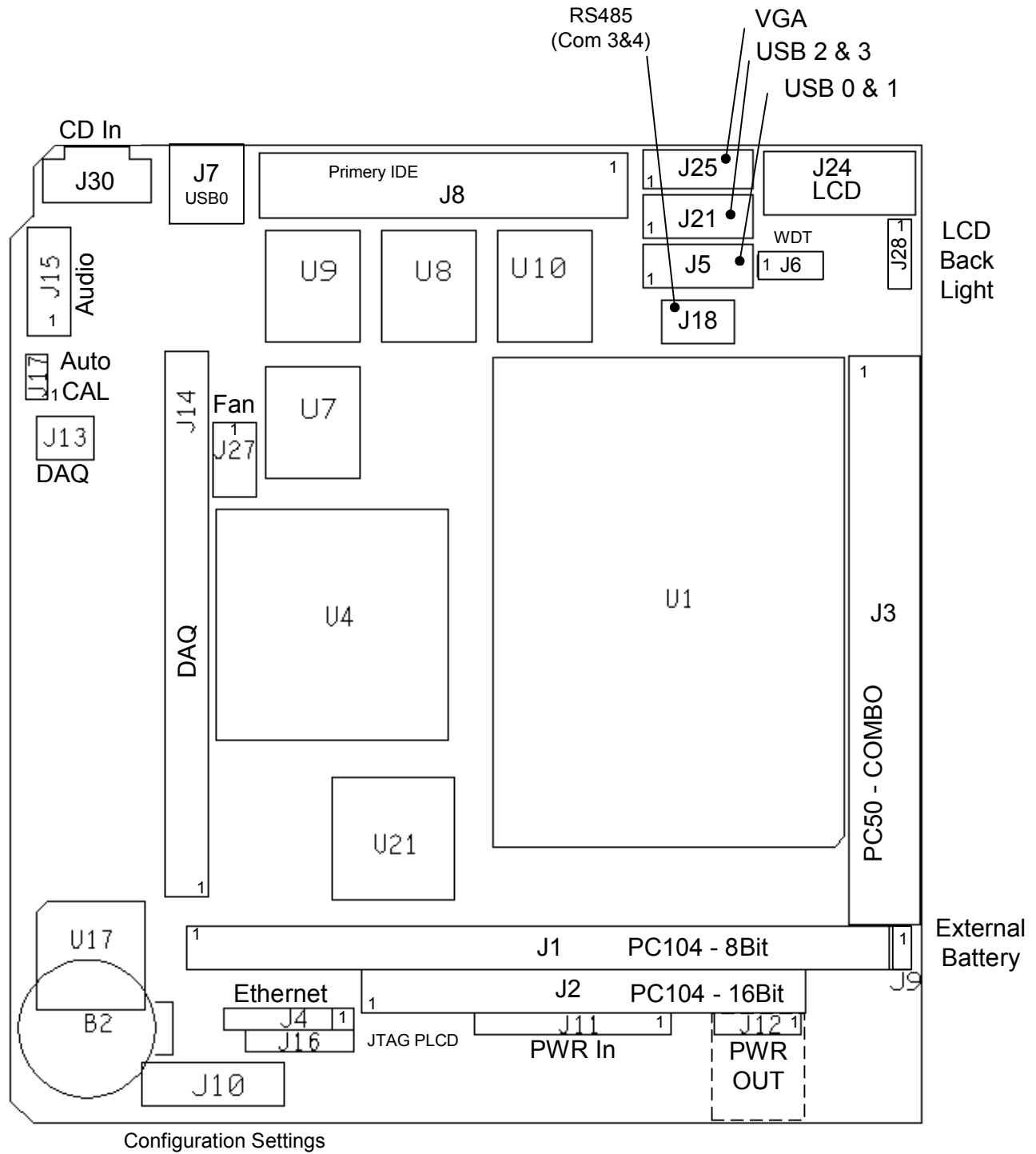
Figure 1. Athena II Connectors
